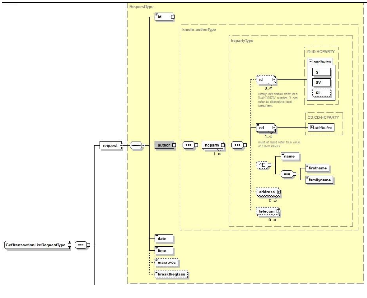
Figure 3: xsd schema: general information
